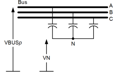
Fig. 3. Ungrounded single-wye bank using neutral voltage unbalance protection.
