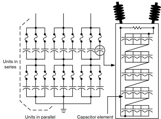
Fig. 1. Typical substation installation of shunt capacitor bank.
