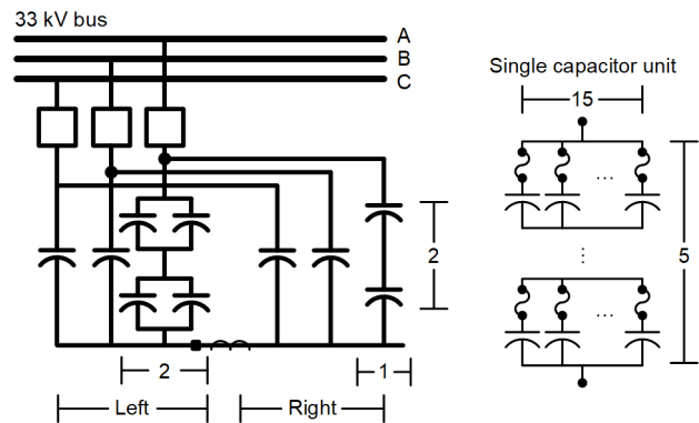
Fig. 10. Capacitor bank model for neutral voltage and neutral current unbalance fault location.
