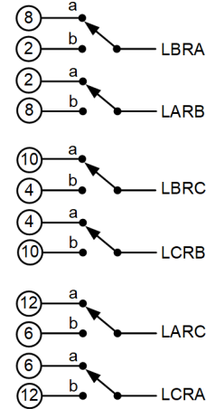
Fig. 6. Multiphase, multisection fault location for ungrounded double-wye banks that use neutral current unbalance protection.
