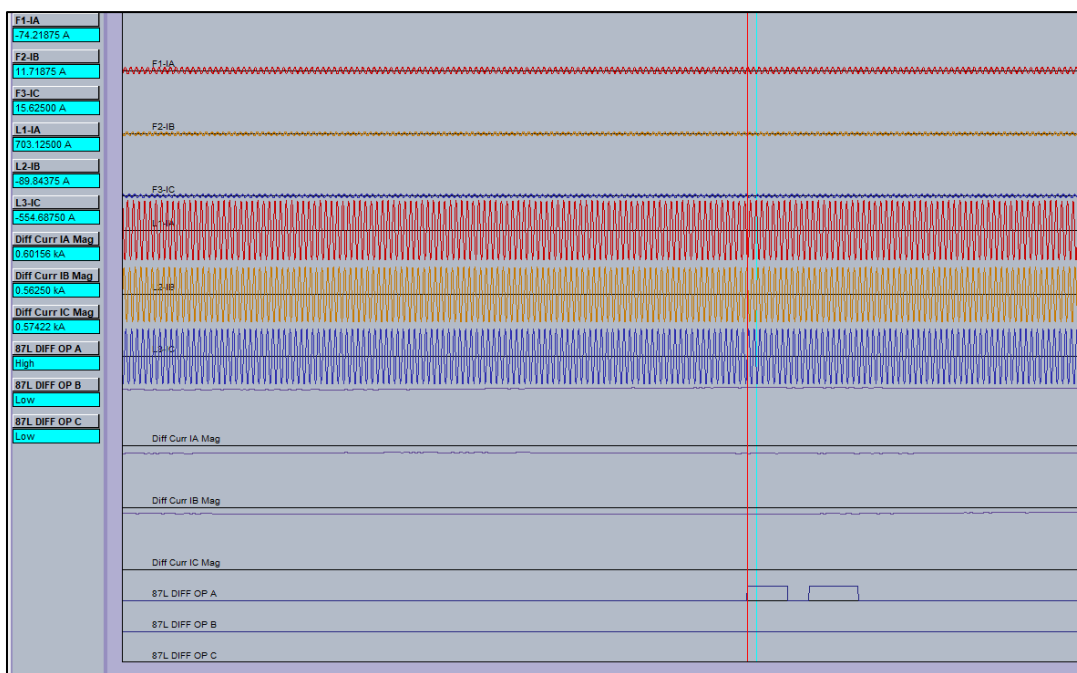
Figure 3 – 87L Line Protection Operation Due to Excessive Channel Asymmetry
