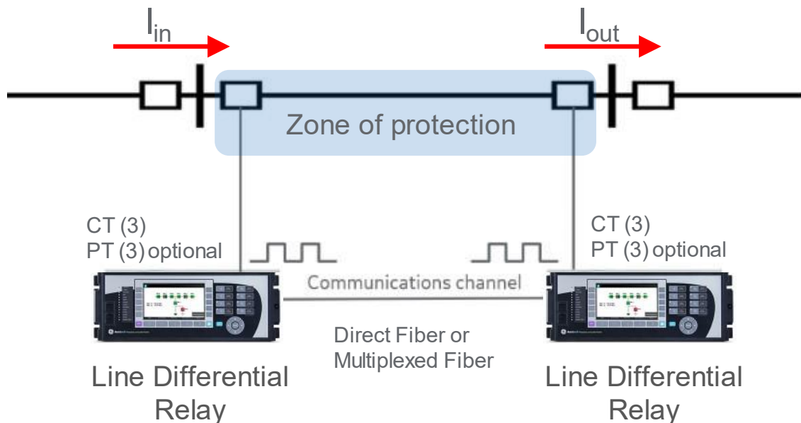
Figure 1 – Two Terminal 87L Transmission Line Protection
