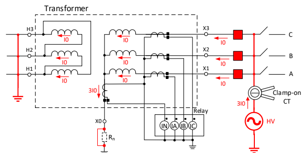
Fig. 18 Connections required for primary injection when terminal or ground CTs are located inside the transformer.
