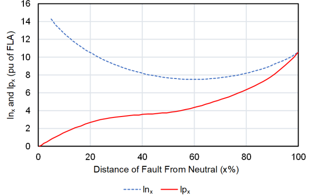
Fig. 5 I_{n_x} and I_{p_x} for ground faults along the winding of a solidly grounded transformer with TR = 1 [9].
