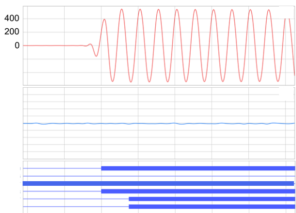
Fig. 17 REF element detects ground fault and asserts within 1.5 cycles.
