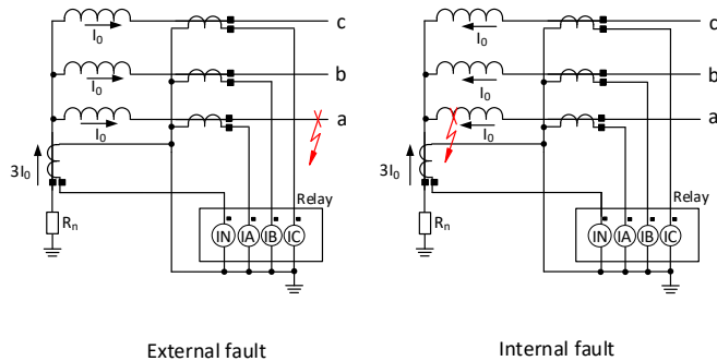
Fig. 8 Ground fault current flow in the wye winding for external (a) and internal (b) faults.
