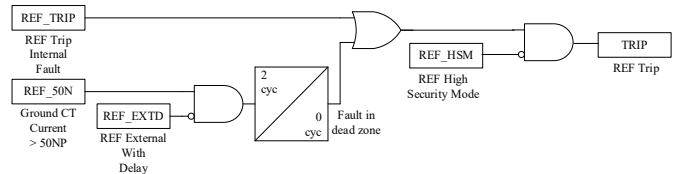
Fig. 14 Using logic to increase the dependability of the traditional REF element when the relay provides REF_EXTD.
