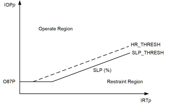
Fig. 2 A simple percentage-restrained differential characteristic.
