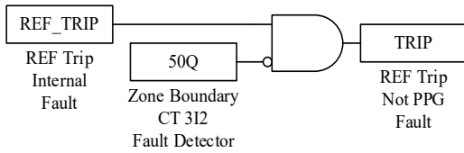
Fig. 11 Adding 50Q supervision for CT saturation on low-impedance grounded systems.
