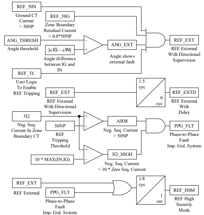
Fig. 10 REF high-security mode logic.
