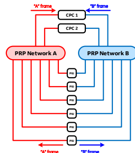
Figure 9: PRP networks
