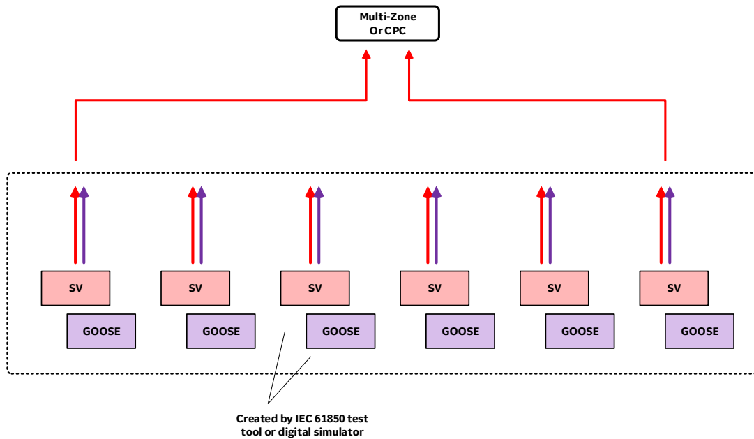
Figure 14: Testing Multi-zone relay/CPC
