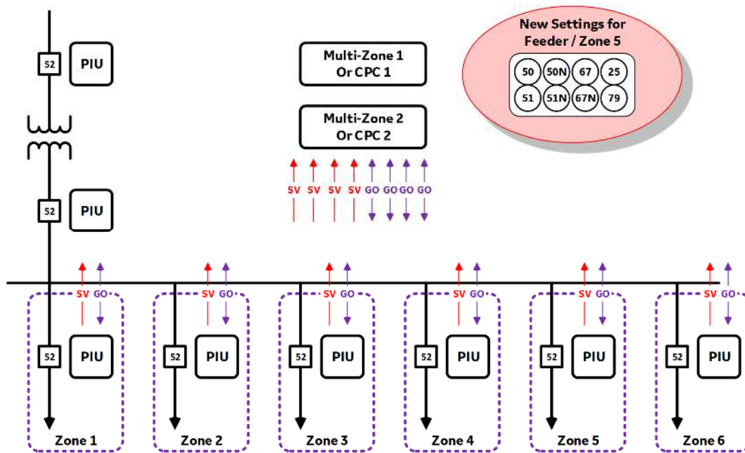
Figure 18: Verifying settings changes in a multi-zone relay/CPC unit
