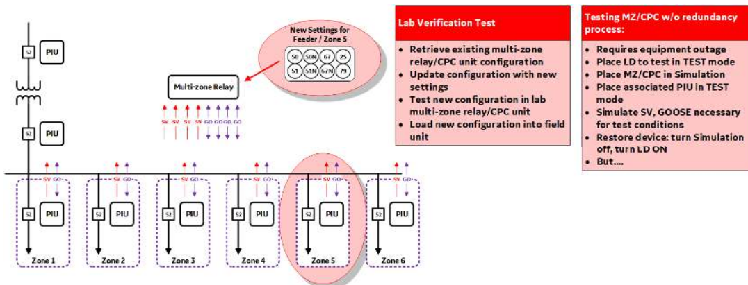
Figure 21: Testing with a single multi-zone relay/CPC unit
