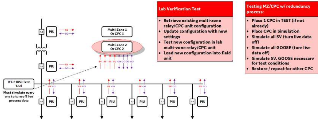
Figure 20: Testing a redundant multi-zone relay/CPC substation
