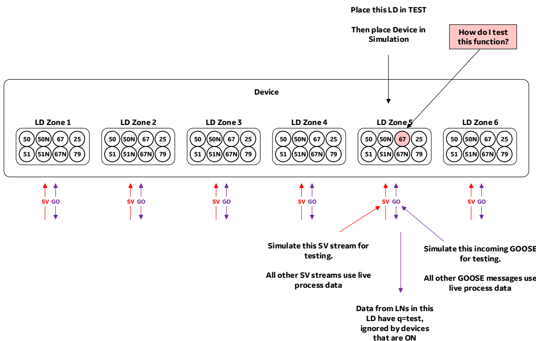
Figure 22: Testing a single LD
