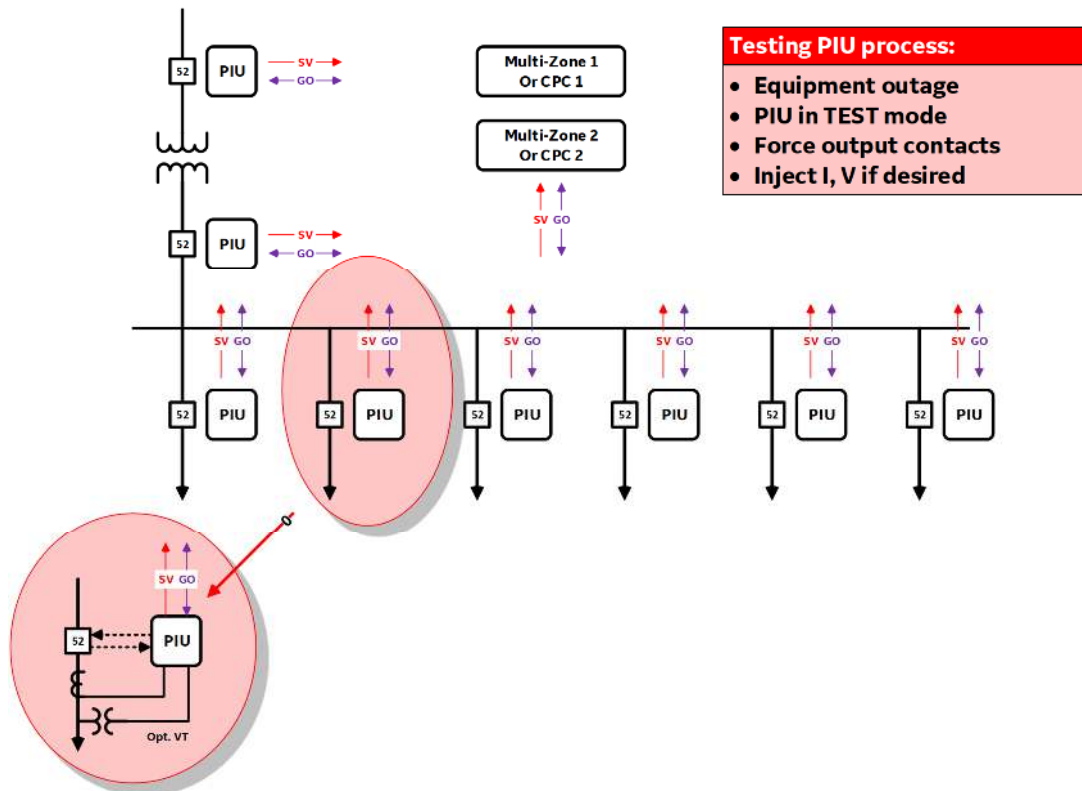
Figure 17: Testing a PIU
