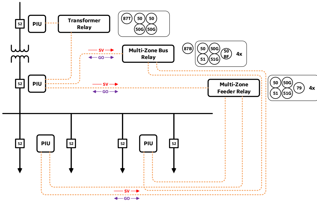
Figure 3: Distribution substation with multi-zone relays
