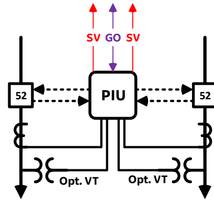
Figure 7: PIU shared between feeders
