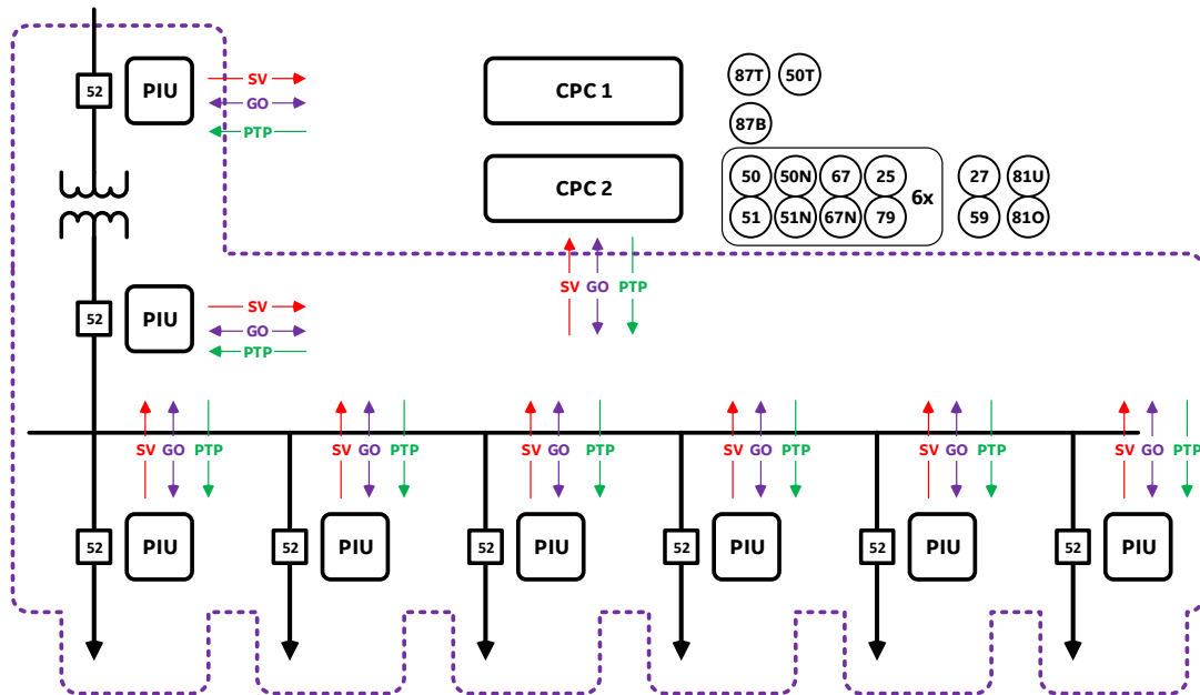
Figure 4: CPC system
