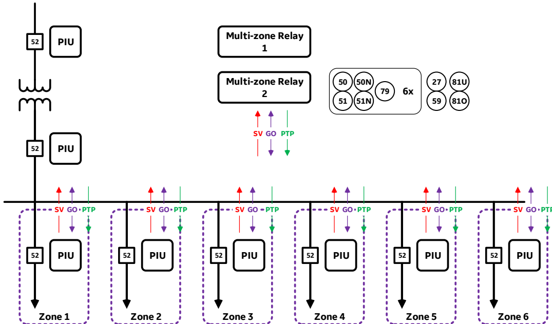
Figure 1: Multi-Zone Protective Relay
