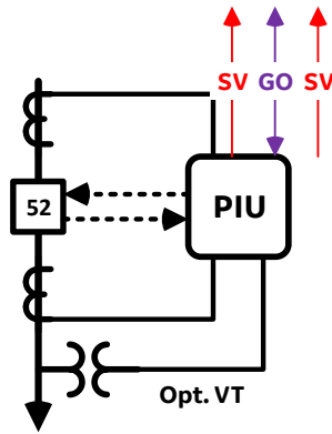
Figure 6: PIU with 2 measurements
