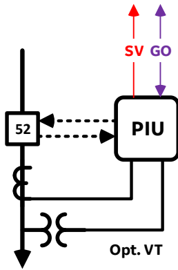
Figure 5: PIU concept
