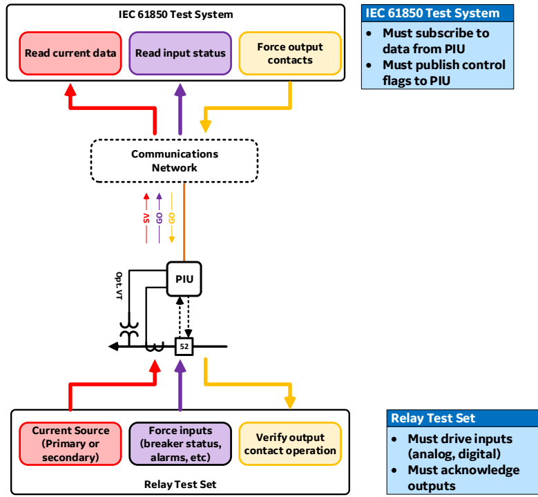
Figure 13: Testing a PIU
